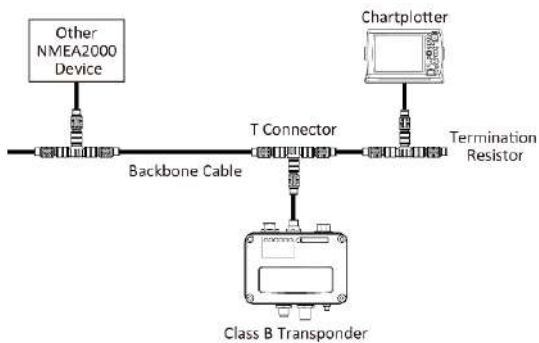
Figure 8 NMEA2000 Network
